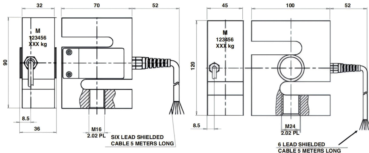
1500, 2000 kg cell outline
